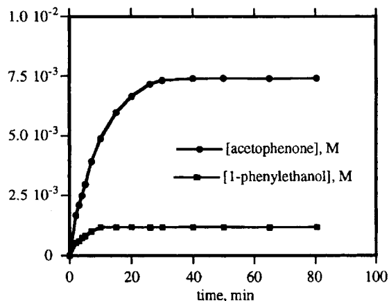
Figure 1. Appearance of the products as a function of time in the oxidation of 0.6 M ethylbenzene with 2.0 \times 10^{-2} M \text{Ph}_4\text{P}(\text{SO}_3)_2 catalyzed by 6.0 \times 10^{-3} M \text{Mn}(\text{TMP})\text{Cl} in the presence of 2.7 \times 10^{-3} M 4- tert -butylpyridine in DCE at 30°C
